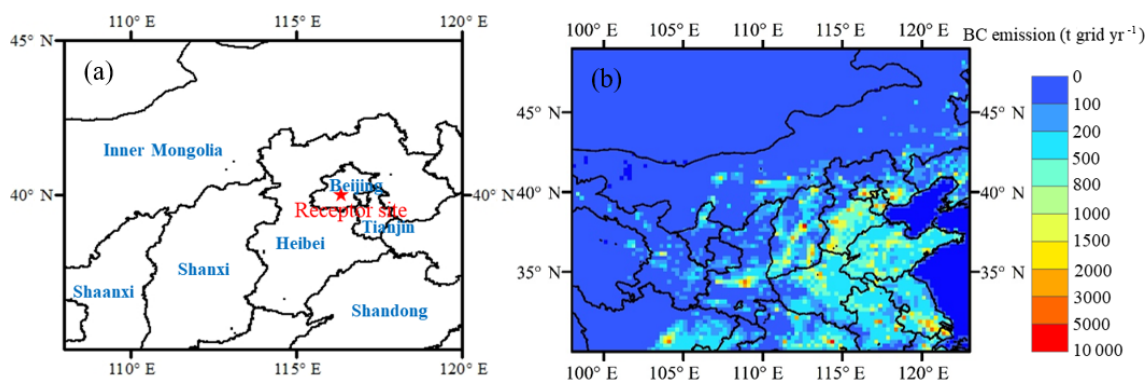
Figure 2. (a) The location of the receptor site (Tsinghua site (40°00′17″ N, 116°19′34″ E), marked as a red star) during the BJNOV2014 measurement period. (b) Spatial distribution (0.25° × 0.25°) of the BC emission inventory from MIX.
