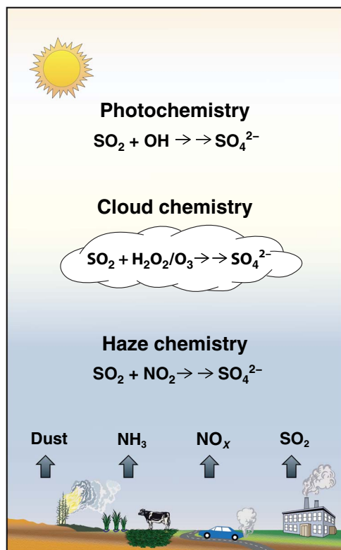
Fig. 4. Conceptual model of sulfate formation in haze events in NCP. The traditional OH, H 2 O 2 , and O 3 reaction pathways in atmospheric gas phase and cloud chemistry are included here, as well as the NO 2 reaction pathway in aerosol water with elevated pH and NO 2 concentrations proposed in this study.
